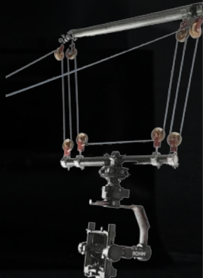
VERTICAL CABLECAM FOR RONIN & MOVI + MIMIC
